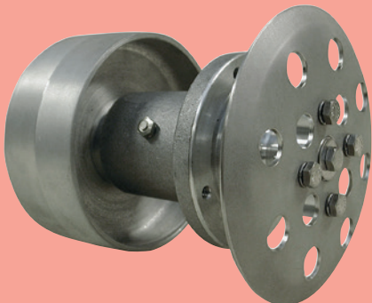
Complete bearing unit with pulley and 12 hole finger disc
