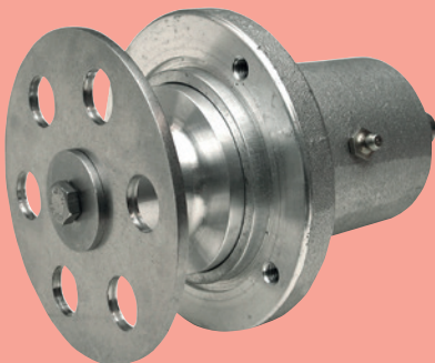
Complete bearing unit with 6 hole finger disc
