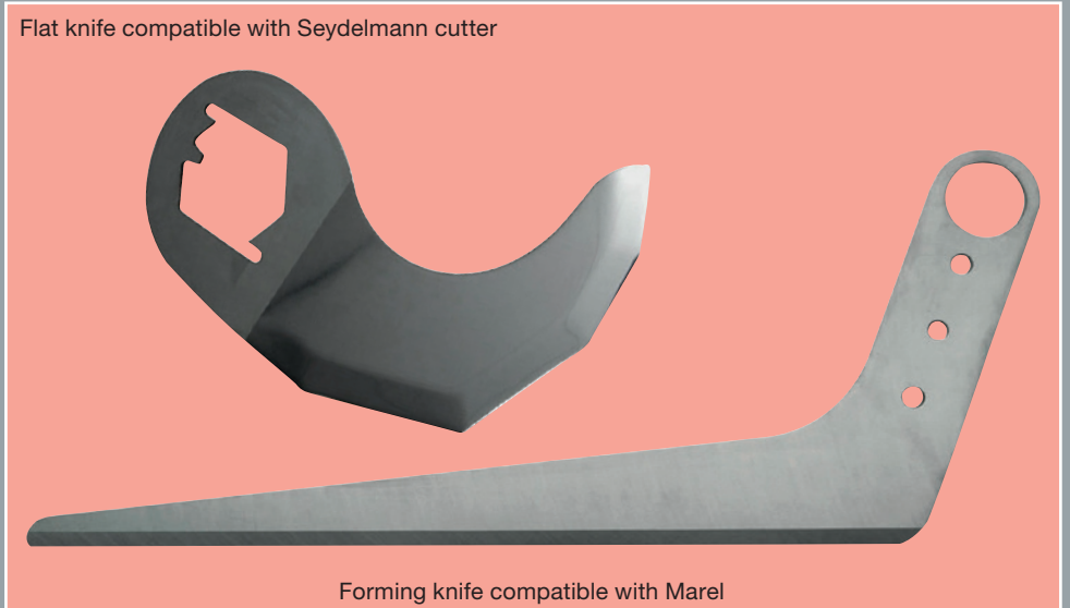
Special shape knives for cut-up systems
